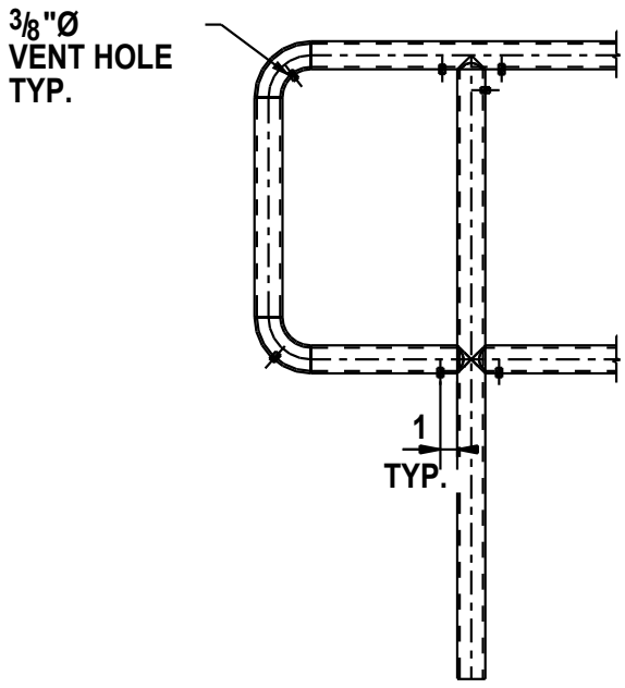
TYPICAL VENT HOLE DETAIL
