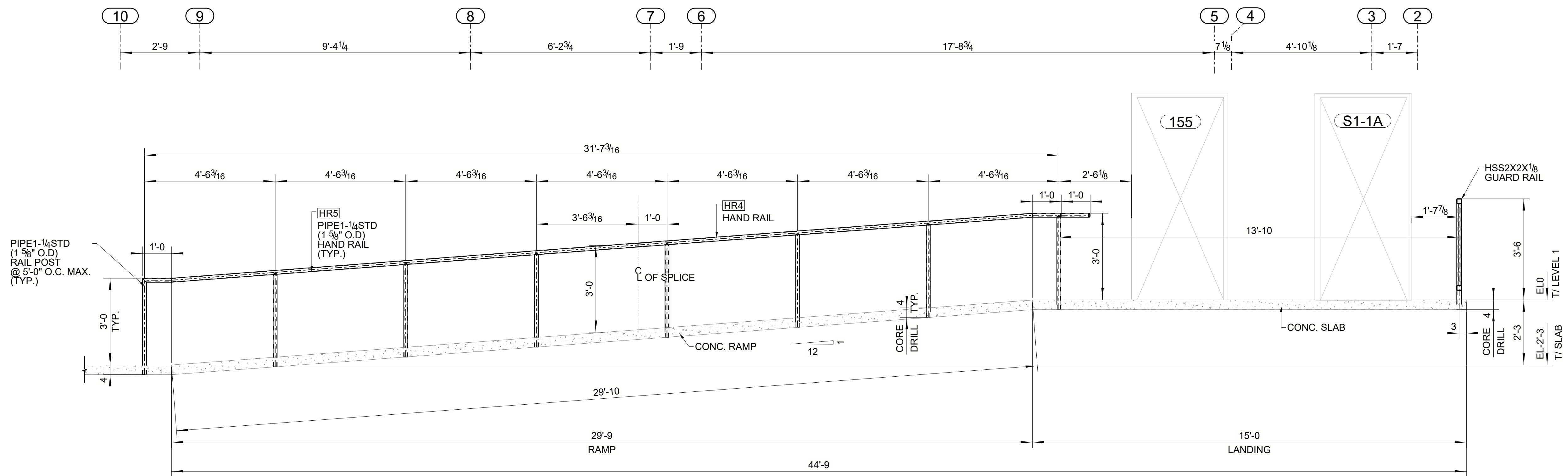
SECTION D - D ME3
