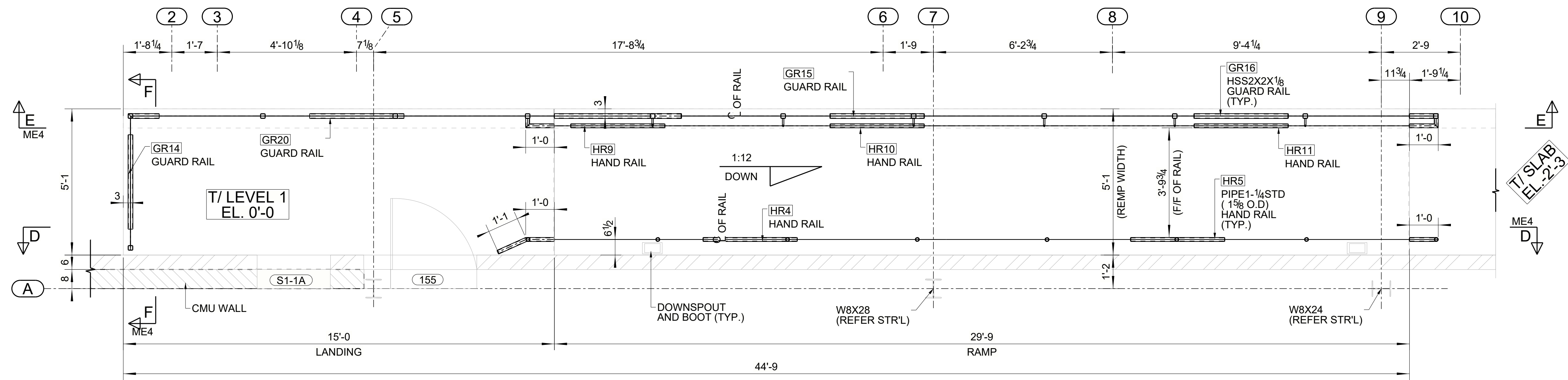
RAMP RAIL LOCATION PLAN (REFER : COMPOSITE FLOOR PLAN- FIRST FLOOR- A2.10 & RAMP PLAN-8/ A8.01)
