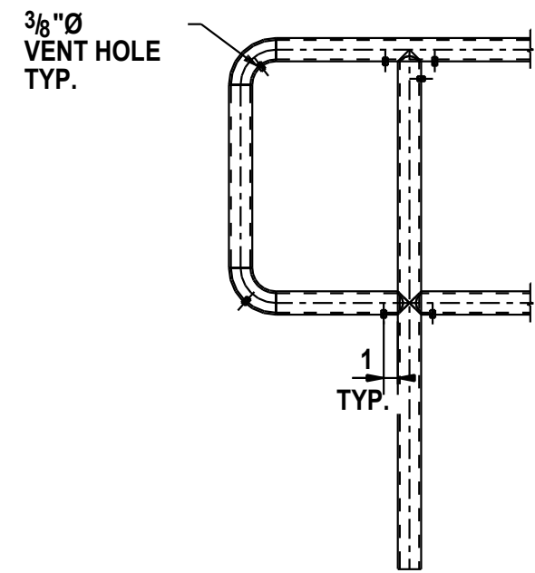
TYPICAL VENT HOLE DETAIL
